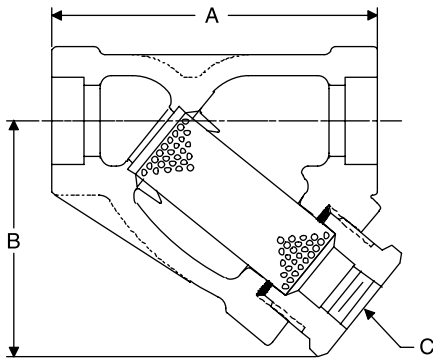
E7SC/E7SW 1/2", 3/4", 1"
